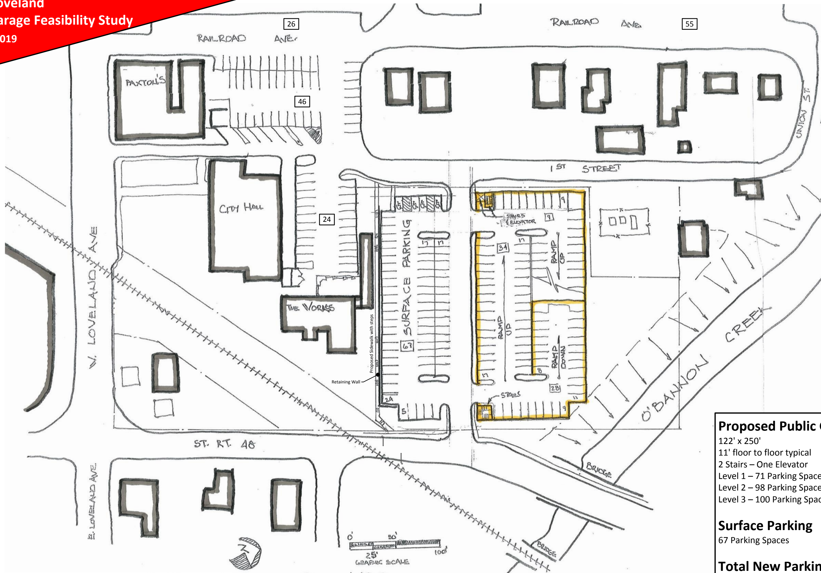
Concept Site Plan No. 2
