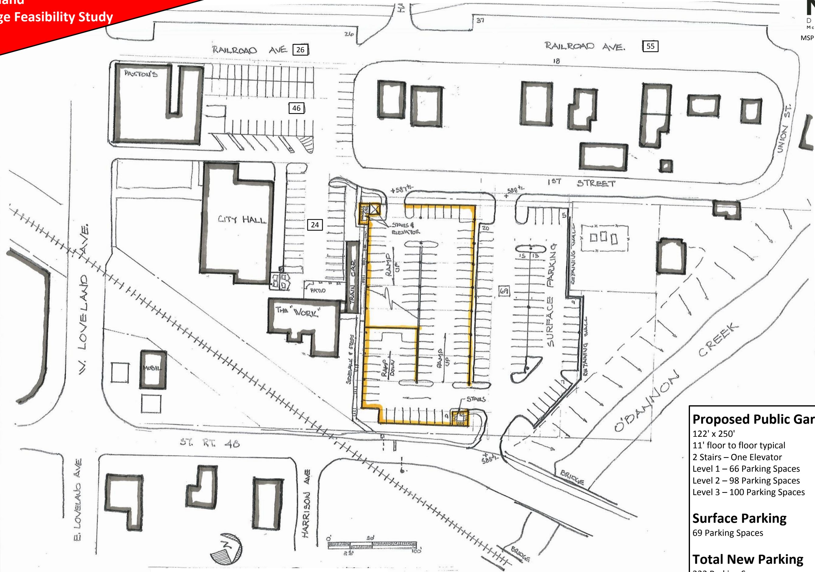
Concept Site Plan No. 1
